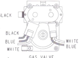
GAS VALVE
